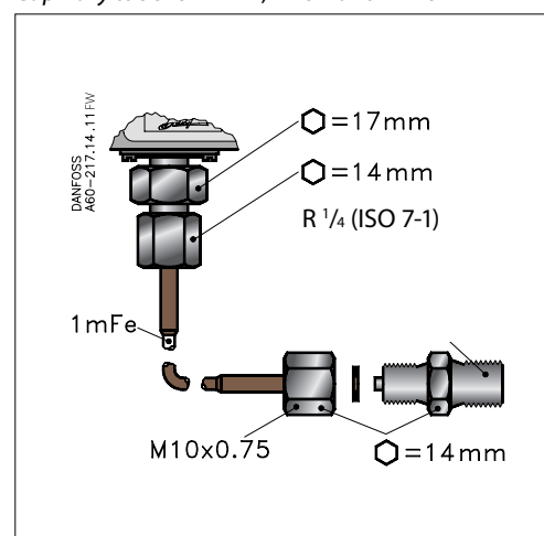
Capillary tube for KP 1A, KP 5A and KP 15A
