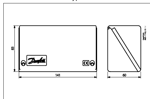
IP55 enclosure for dual types
