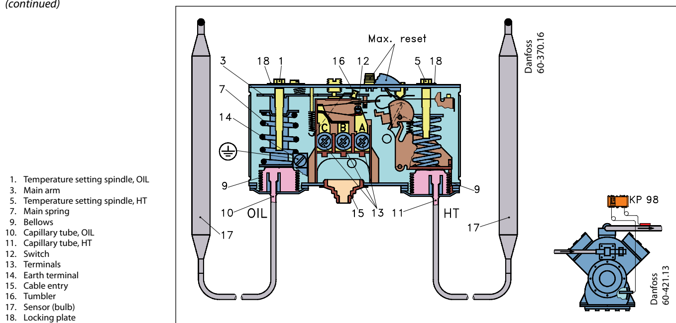
KP thermostat, dual type
